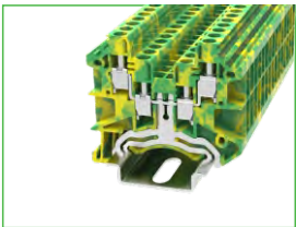
DC4-QU-PE (Cross & Slotted screw)
