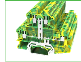
DCKKB2.5-PE-02A(H) (Cross & Slotted screw)
