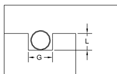
Quick-Shield in an o-ring groove.
