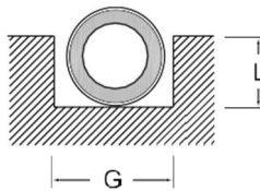
Flexi-Shield mounted in standard o-ring groove.
