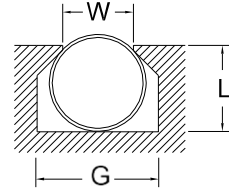
dovetail groove
