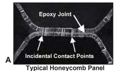
Microscopic Photos of Honeycomb Panel Cells
