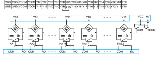
DM108-RMS-32-PN-1-4M-00Z(H)
