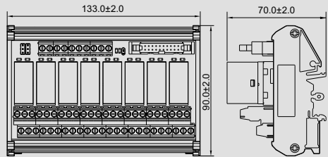
DM72-RM-08-PN-4-4M-10Z(H)
