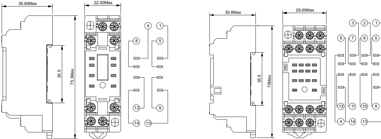
DPYF08A-E3
