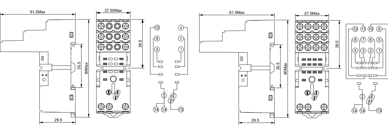
DPKF08A-F3
