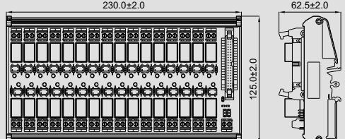
DM108-RMS-32-PN-1-4M-00Z(H)
