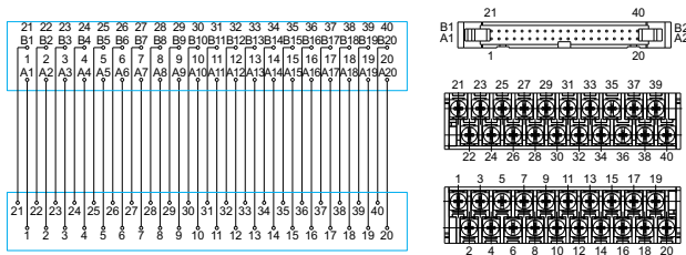
DM50-IDC-40-40-4G-00Z(H)
